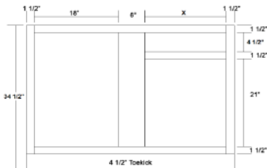
Opening Width Calculation Cabinet Width - 27" = X
