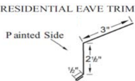
RESIDENTIAL EAVE TRIM
