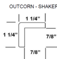
OUTCORNSHAKER
