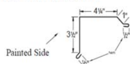
RESIDENTIAL RAKE
