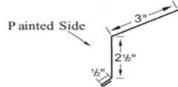
RESIDENTIAL EAVE TRIM
