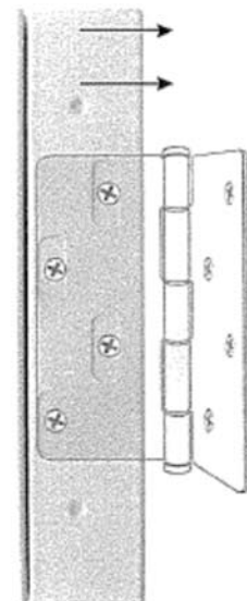
Fig. 6 Out Adjustment
