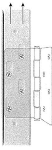
Fig. 3 Up Adjustment
