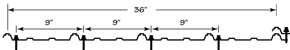
Fastener Pattern at Interior of Panel
