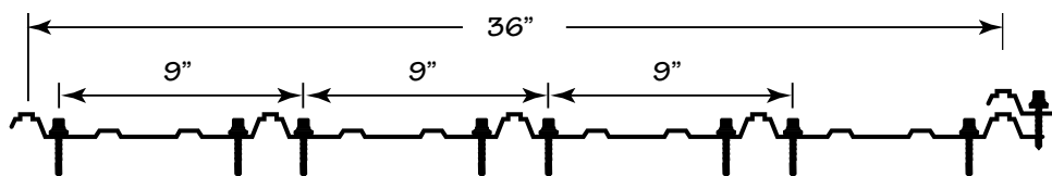
Fastener Pattern at Eave and Endlap
