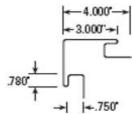
UNIVERSAL INSIDE CORNER MATTE FINISH
